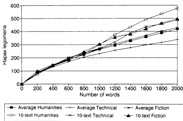
Fig. 7 Distribution of Hapax legomena in texts from three registers
