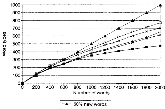
Fig. 2 Distribution of word types in five humanities texts
