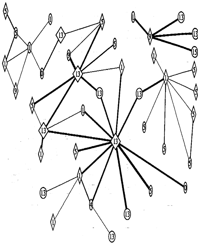
FIGURE 3. Network configuration* for a community group in Atlanta, Georgia, 1995-1999, in which HIV transmission was not known to have taken place. *Numbers are Risk Indicators (see text). Shapes reflect gender: Circles or ovoids are men, and diamonds are women. The thickness of the line represents the kind of contact: The thickest lines represent simultaneous sexual and needle-sharing connections; intermediate lines convey either sex or needle sharing; thin lines reflect neither sex nor needle connections.
