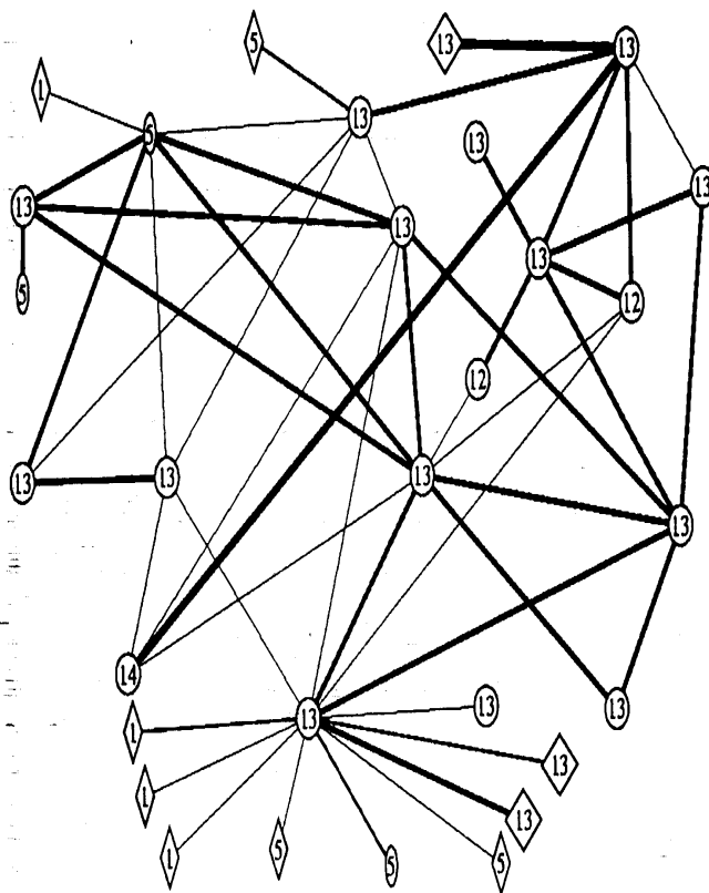
FIGURE 2. Network configuration* for a community group in Atlanta, Georgia, 1995–1999, in which HIV transmission took place. *Numbers are Risk Indicators (see text). Shapes reflect gender: Circles or ovoids are men, and diamonds are women. The thickness of the line represents the kind of contact: The thickest lines represent simultaneous sexual and needle-sharing connections; intermediate lines convey either sex or needle sharing; thin lines reflect neither sex nor needle connections.
