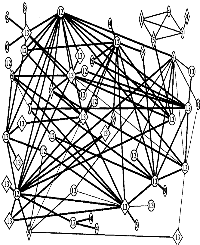
FIGURE 1. Interaction of persons* in a community chain in Flagstaff, Arizona, 1995–1998. *Numbers are Risk Indicators (see text). Shapes reflect gender: Circles or ovoids are men, and diamonds are women. The thickness of the line represents the kind of contact: The thickest lines represent simultaneous sexual and needle-sharing connections; intermediate lines convey either sex or needle sharing; thin lines reflect neither sex nor needle connections.
