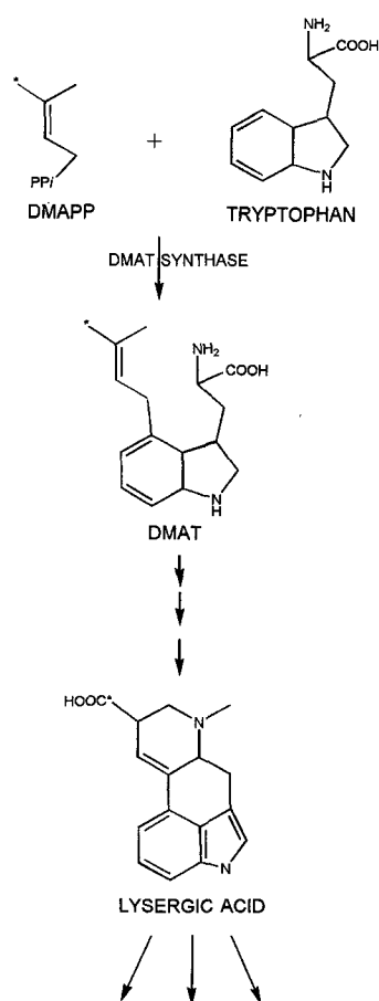
Figure 3. Reaction catalyzed by DMAT synthase in ergot alkaloid biosynthesis. Products of lysergic acid include the simple acids and alcohols, amides, single amino acid derivatives, and complex ergopeptide derivatives such as ergovaline. DMAPP, Dimethylallyl diphosphate.
