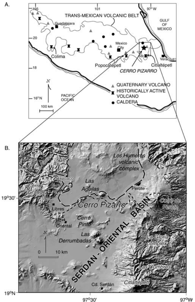
Fig. 1 A Central Mexico showing the Trans-Mexican Volcanic Belt. B DEM image of the Serdán Oriental basin in the eastern Trans-Mexican Volcanic Belt, showing Cerro Pizarro and other volcanoes of the eastern belt. Short dashed line represents likely outcrop areas of the Xáltipan ignimbrite prior to eruption of Cerro Pizarro; long dashed line represents outcrop areas of the Zaragoza ignimbrite; both derived from Los Humeros volcanic complex. Sierra Negra lies just to the south of the image area; La Malinche lies to the west
