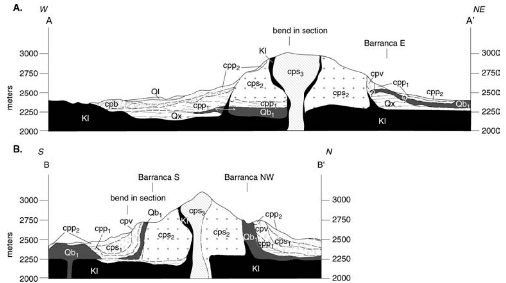
Fig. 5 Cross sections approximately east–west ( A ) and north–south ( B ) through Cerro Pizarro. For locations see Fig. 2B. Symbols as for Fig. 2B, with the addition of Qx, Quaternary Xáltipan ignimbrite
