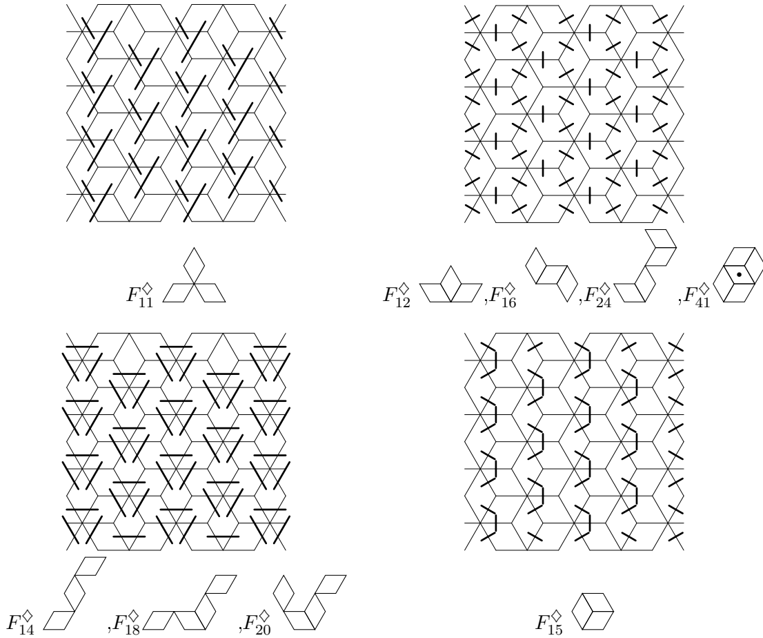
Figure 4.5: Animals and the pavings that kill them.
