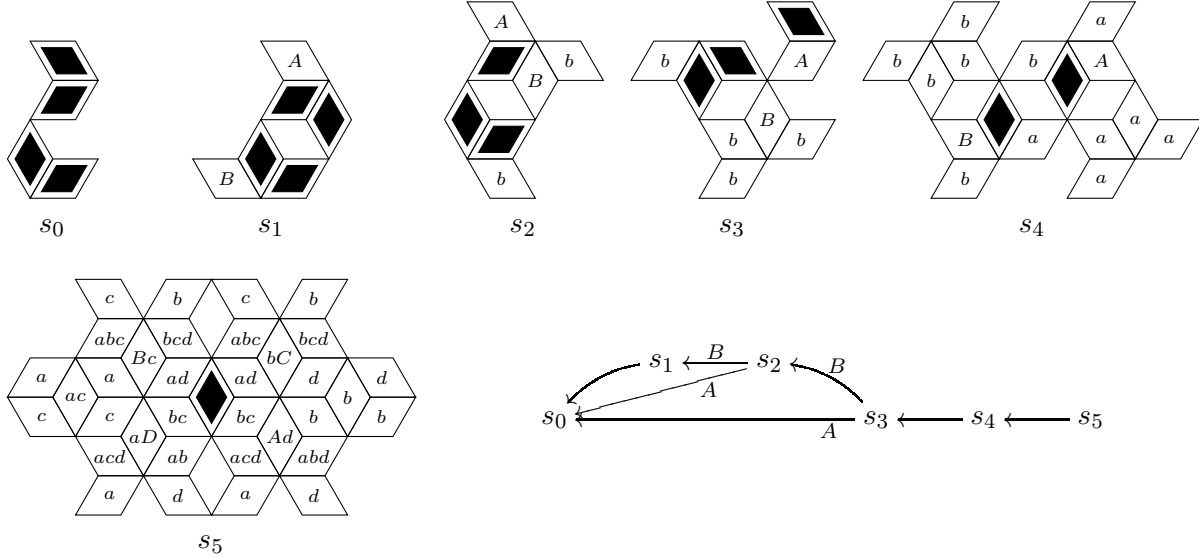
Figure 4.7: A (1,1)-proof sequence for F_{28}^{\diamond} .
