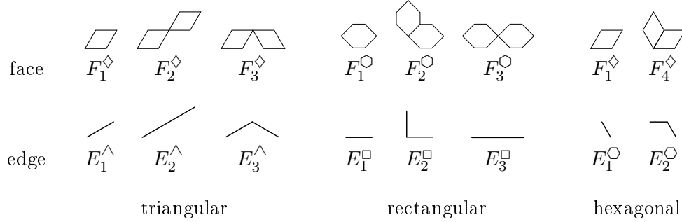
Figure 2.2: Edge animals up to size two and their corresponding face animals. Triangular and rectangular edge animals have wild corresponding face animals. Hexagonal edge animals have regular corresponding face animals.
