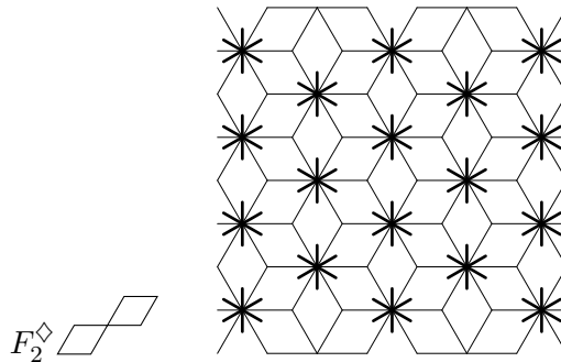
Figure 4.2: The animal F_2^\diamond and the paving that kills it.
