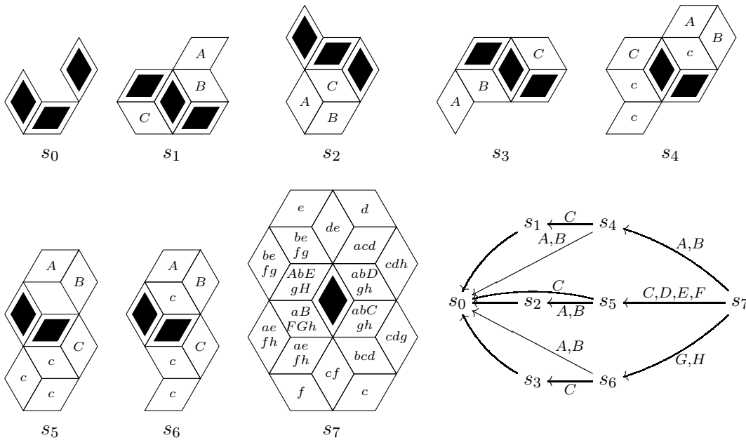
Figure 4.4: A proof series for F_{10}^\diamond .
