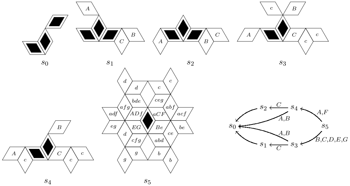
Figure 4.3: A proof sequence for F_9^\diamond .
