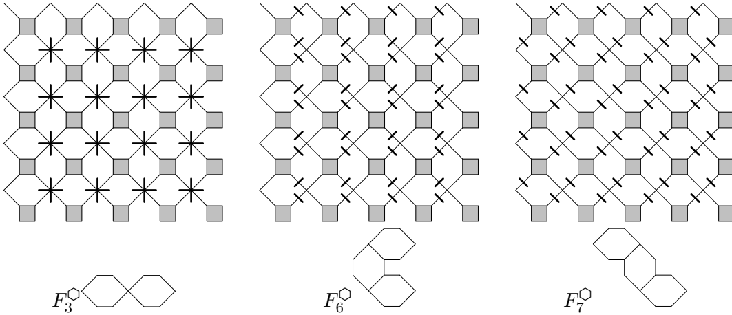
Figure 5.2: Animals and the paving that kills them.
