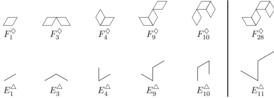
Figure 6.1: Known triangular edge winners and the mystery animal F_{28}^{\diamond} together with their corresponding face animals.
