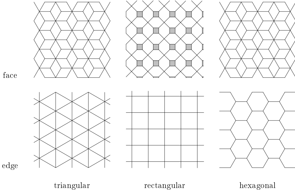
Figure 2.1: Edge boards and their corresponding face boards.
