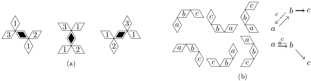
Figure 4.6: (a) The priority strategy for the breaker to prevent the maker from marking F_{13}^\diamond . (b) Dependency digraphs of the cells in the orientations of F_{13}^\diamond .
