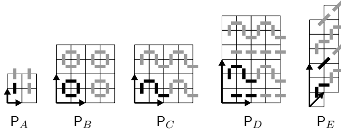
FIGURE 5.1. 2-pavings. Each picture shows four copies of the fundamental set of tiles.
