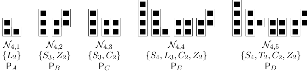
FIGURE 6.6. Characterizing teams for size 4. Killer 2-pavings are listed for losing teams. No winning team is required.
