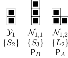
FIGURE 6.1. Characterizing families for size 1. Killer 2-pavings are listed for losing families.
