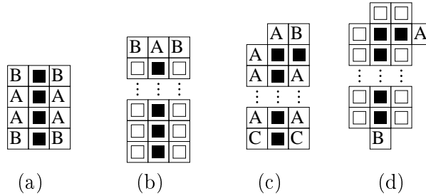
FIGURE 4.2. Situations to achieve \mathcal{W}_n .
