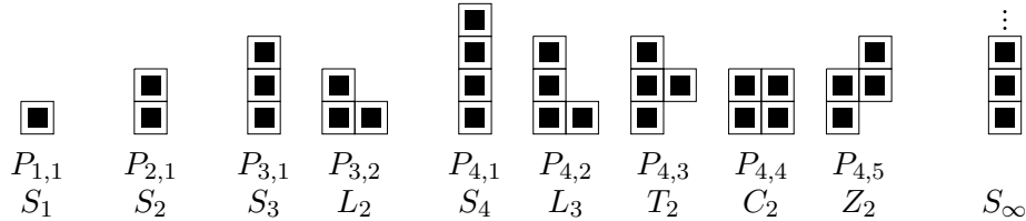
FIGURE 2.1. All polyominoes up to size 4 together with infinite skinny.
