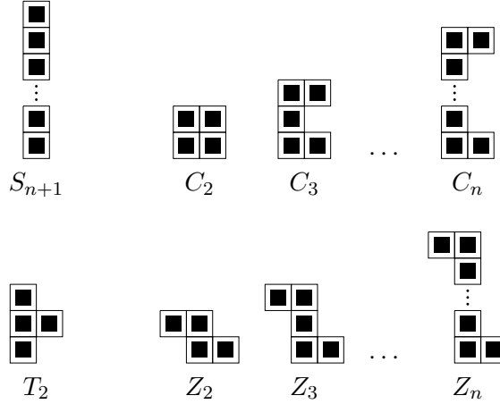
FIGURE 4.1. The winner \mathcal{W}_n .
