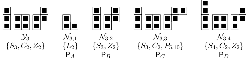
FIGURE 6.3. Characterizing families for size 3. Killer 2-pavings are listed for losing families.
