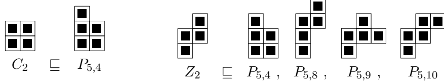
FIGURE 6.4. Descendants of C_2 and Z_2 with size 5 .
