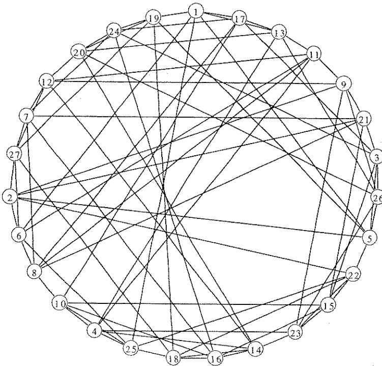
Figure D: An example of a primitive graph.
