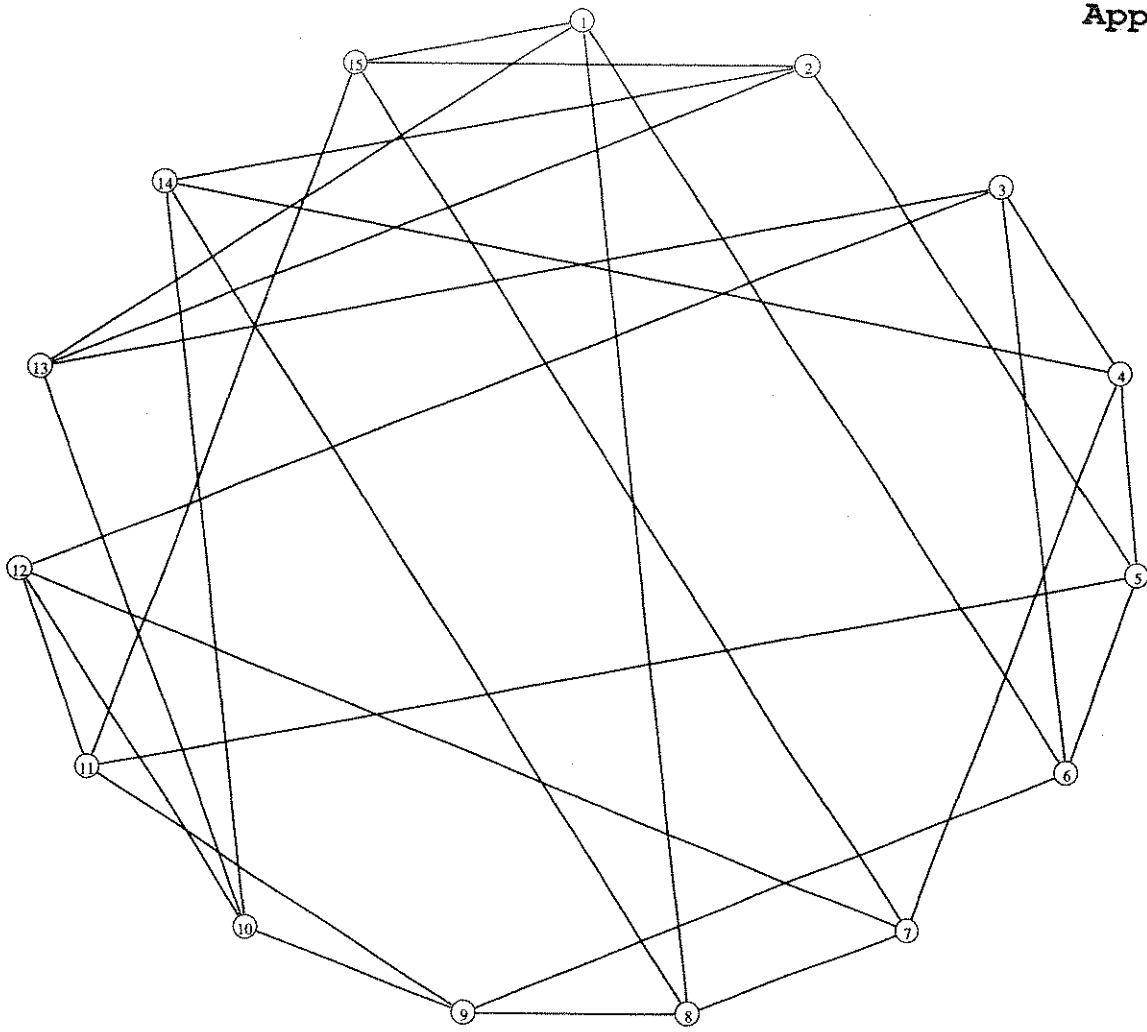
Graph: Appendix I
