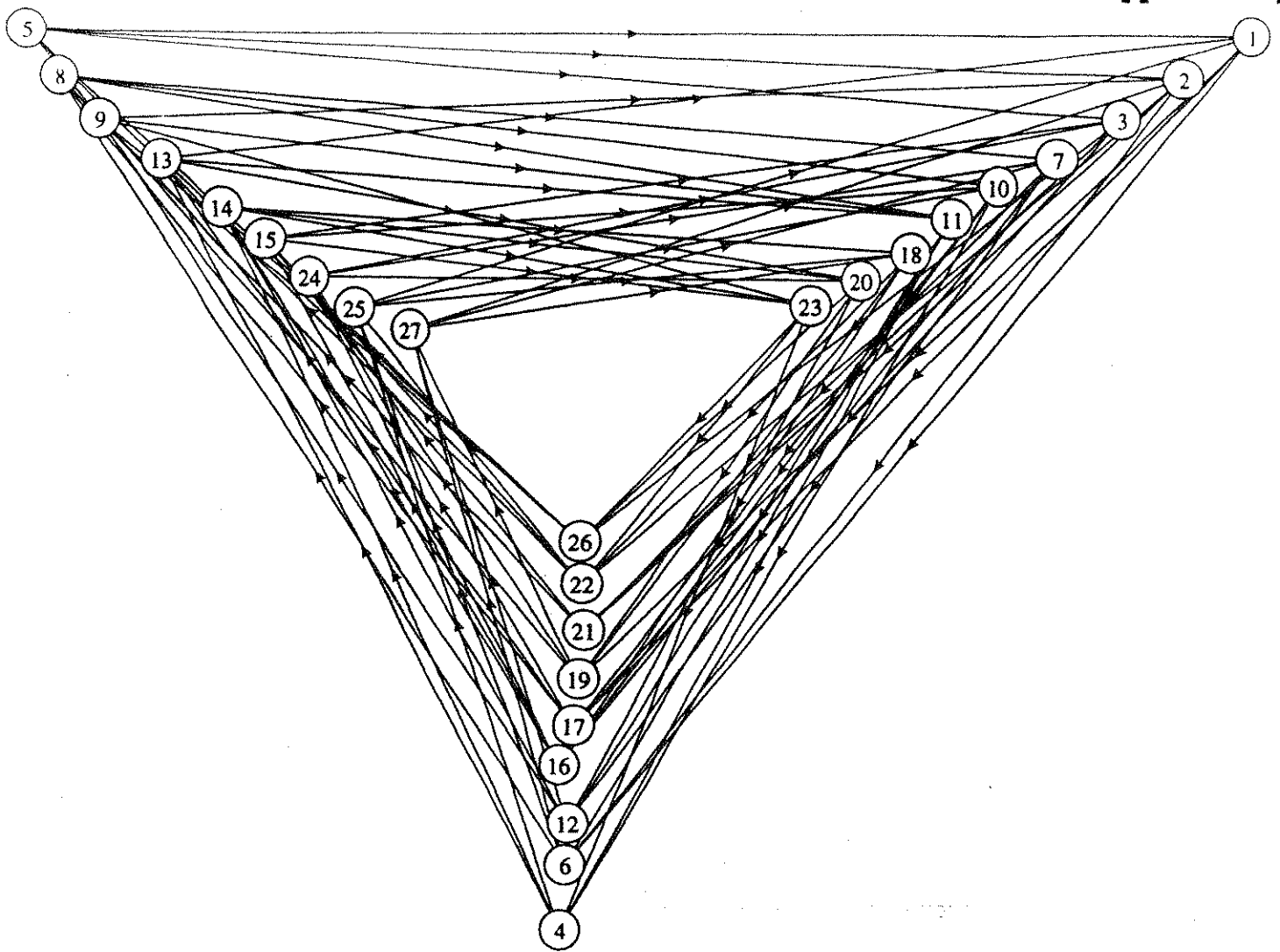
Digraph: Appendix Q
