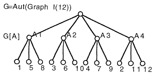
Figure F: Block for Figure E
