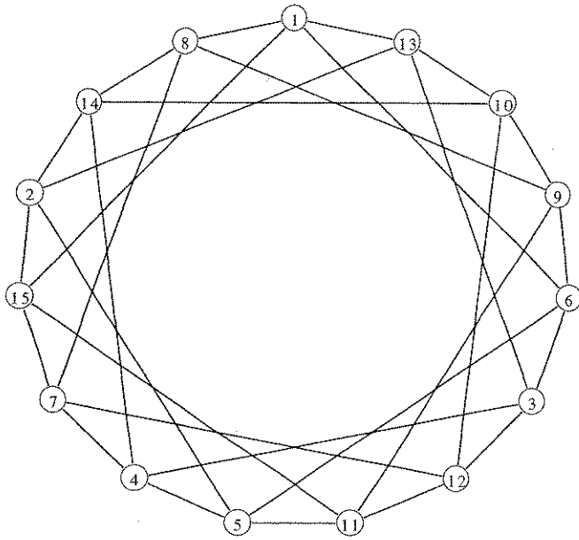
Figure A: C_{15}(1,4)
