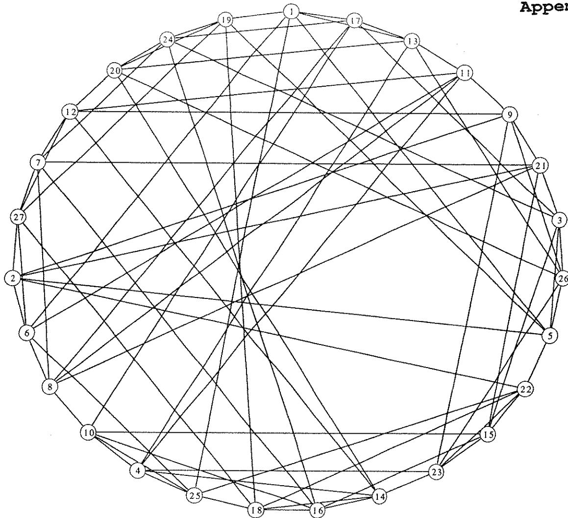
Graph: Appendix M
