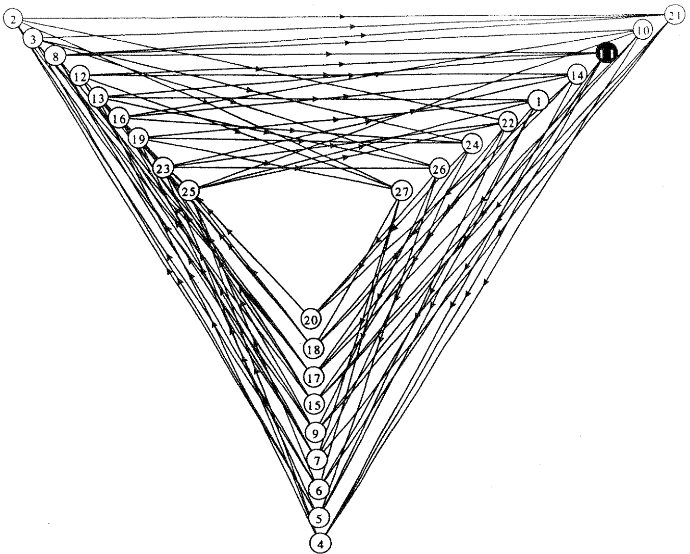
Digraph: Appendix S
