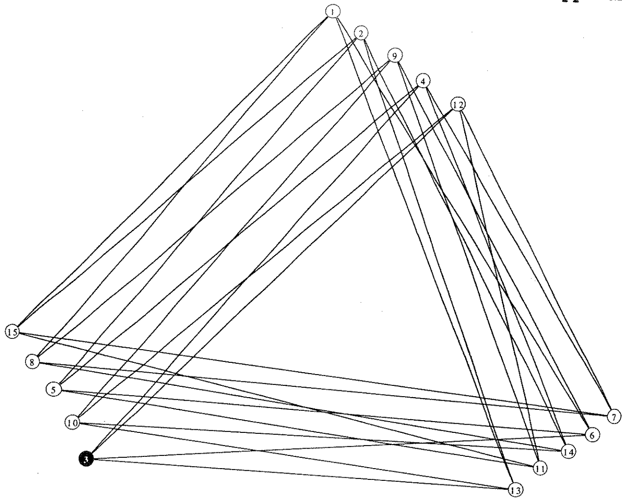
Graph: Appendix L 15 Vertices, 30 Edges
