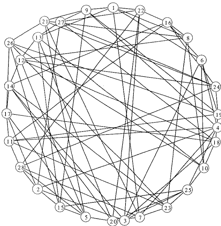
Figure B: 28 Vertices, 84 Edges
