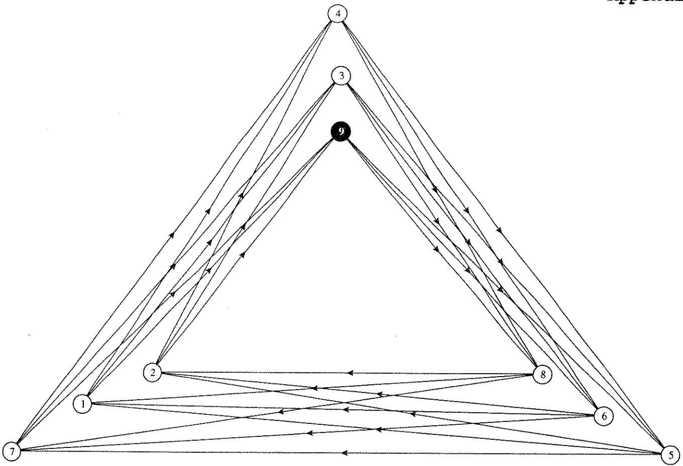
Digraph: Appendix A
