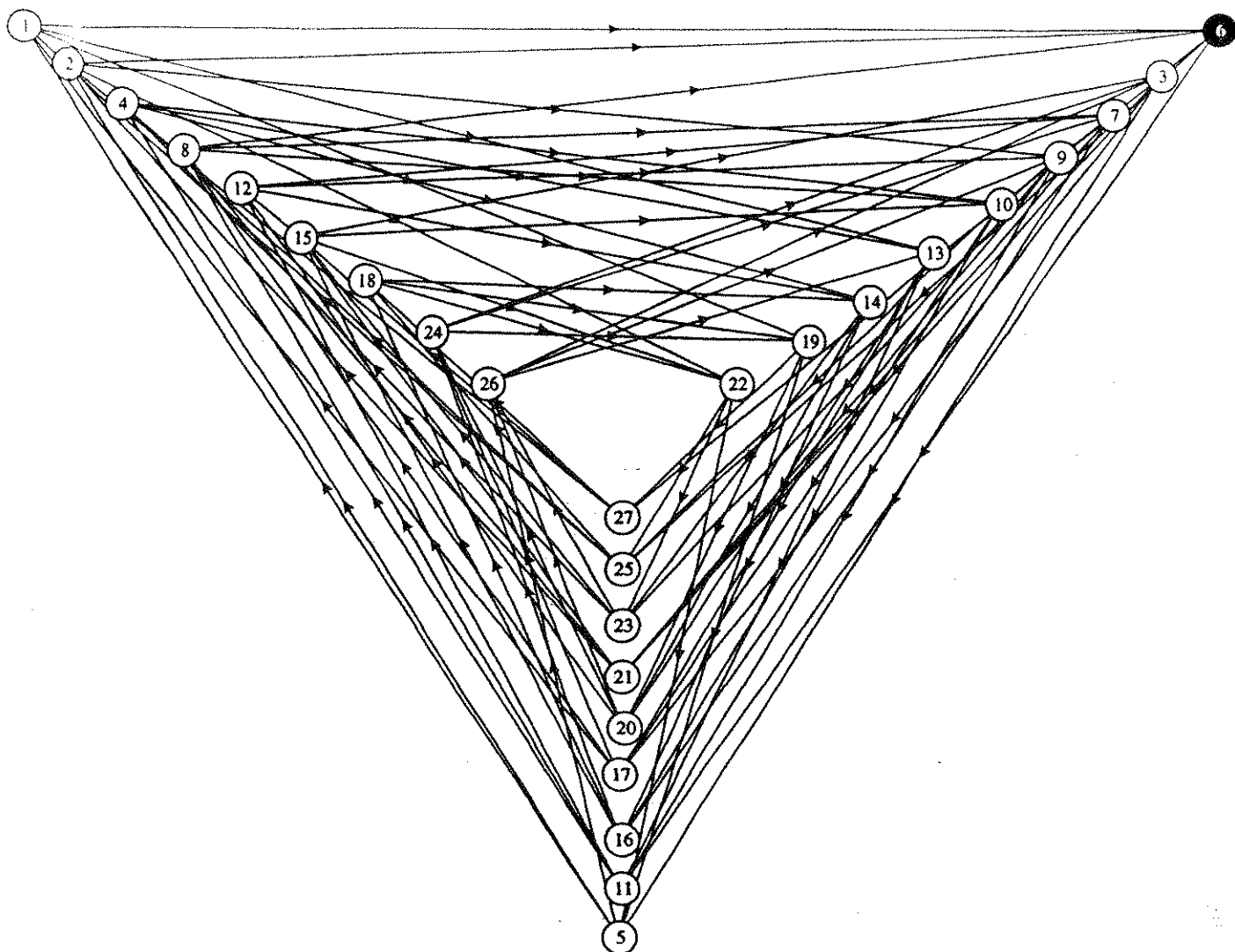
Digraph: Appendix P
