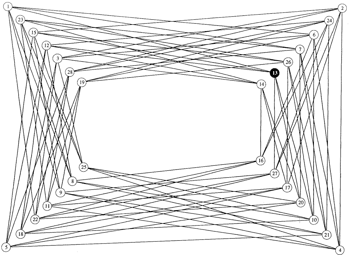
Graph: Appendix C
