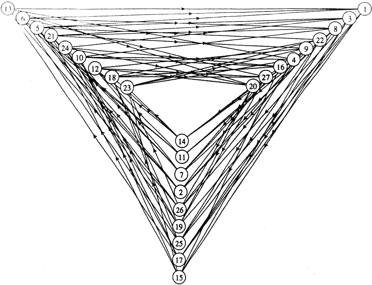
Digraph: Appendix R
