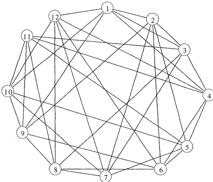
Figure E: An imprimitive graph
