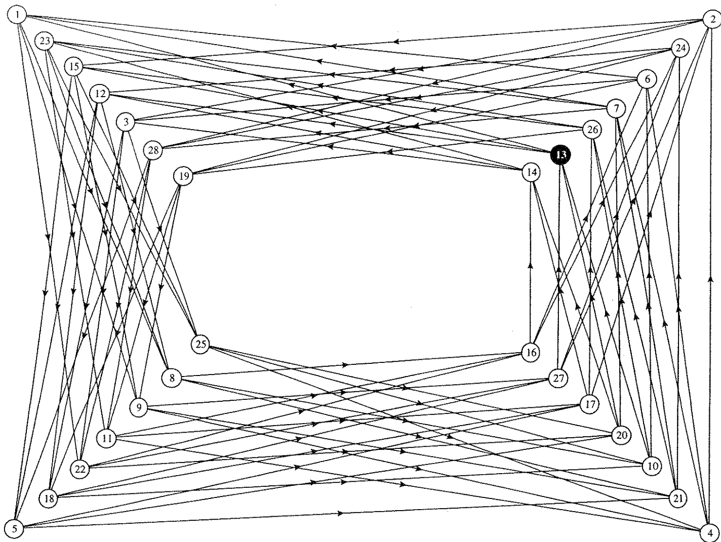
Digraph: Appendix D
