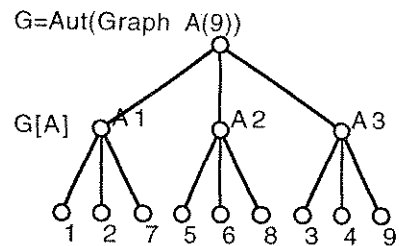
Figure D: Block for Figure C
